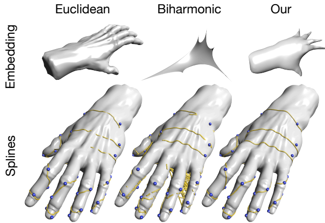
Figure 8: Top: The original surface (Euclidean embedding) and the first three dimensions of the biharmonic embedding and our embedding for the hand mesh. The biharmonic embedding tends to collapse thin features, making it unsuitable for weighted averages computations on these regions. Bottom: Cubic B-splines using different Euclidean-embedding metrics. Discontinuities in the weighted averages computed with Euclidean and Biharmonic embeddings can be seen as both the yellow curve passing through the surface (to connect to a far-away point) and as artifacts on the fingers. All of these results were computed using Phong projection.
