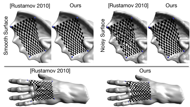
Figure 10: The inverse problem with four anchors defines a mapping from mesh vertices onto a checkerboard, which is used as a texture. For a smooth mesh, our method and Rustamov’s [2010] perform similarly, but when the mesh is corrupted by a small amount of noise, our metric is more robust than exact geodesic distance. The symmetrized L^2 stretch [Schreiner et al. 2004] of the mapping on the smooth wing is slightly worse with our method (0.75 compared to 0.88 for [Rustamov 2010]), the ideal measure being 1. Similarly for the hand, our mapping has a stretch of 0.74 compared to 0.83.
