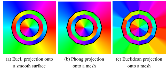
Figure 6: Comparison of the qualitative behavior of (a) projection onto a smooth surface, (b) Phong projection, and (c) Euclidean projection onto a mesh. The smooth surface is a torus, which is discretized in (b) and (c). Each image shows a plane through the center of the torus; each point is colored based on the angle between the vector from that point to its projection and the x -axis. Phong projection behaves similarly to projecting onto the smooth torus, while Euclidean projection shows clear discontinuities.
